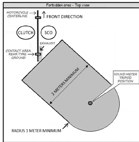
Figure 8 : Prohibited area during the Sound Control
