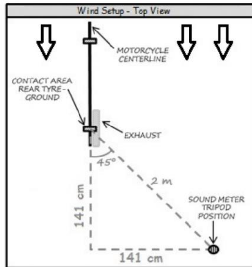
Figure 7 : Setup during windy conditions
