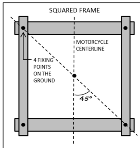
Figure 6 : Squared frame design
